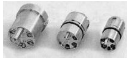
From left to right: PRO BEAM Sr., PRO BEAM Jr. & PRO BEAM Mini Expanded Beam inserts.
